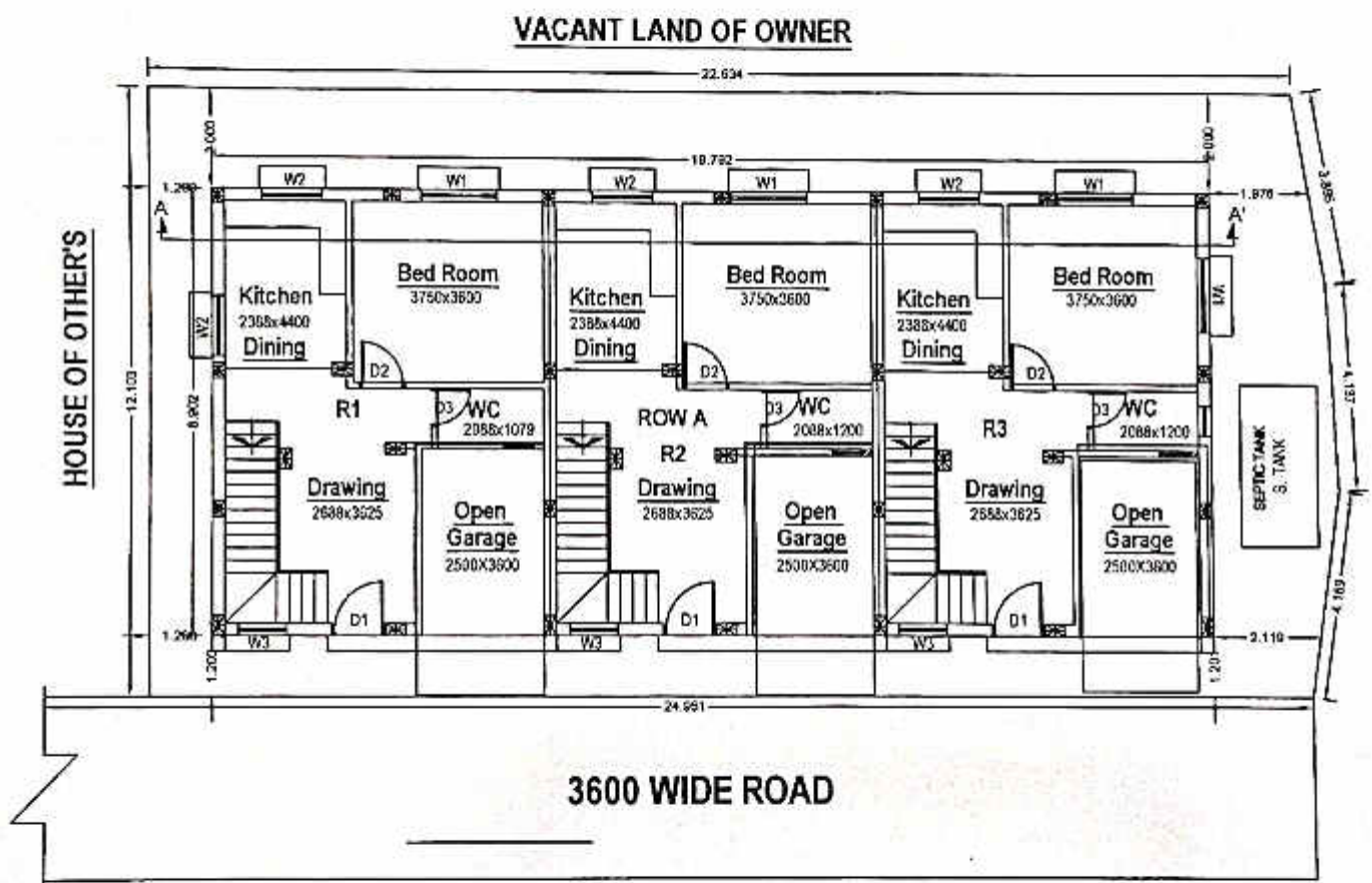
SITE PLAN WITH GROUND FLOOR PLAN
